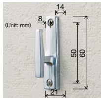
Tieback Hook / Type F (Silver)
