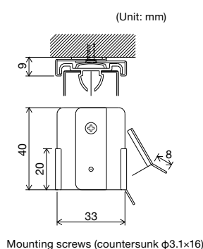
Mounting screws (countersunk \phi 3.1 \times 16 )
