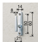
Tieback Hook Type F (Silver)
