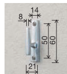
Tieback Hook Type F (Silver)
