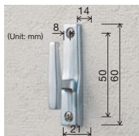
Tieback Hook / Type F (Silver)
