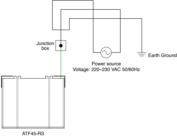
Basic Connecting Diagram
