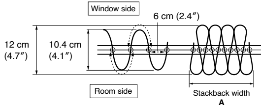
Wave Style Composition of 2.0 Times Fullness
