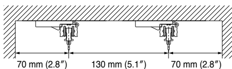
Installation Dimension of 2.0 Times Fullness (example for New Delac)
