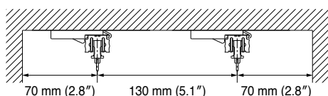
Installation Dimension of 1.5 Times Fullness (example for New Delac)
