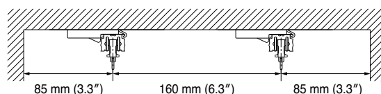
Installation Dimension of 1.875 Times Fullness (example for New Delac)
