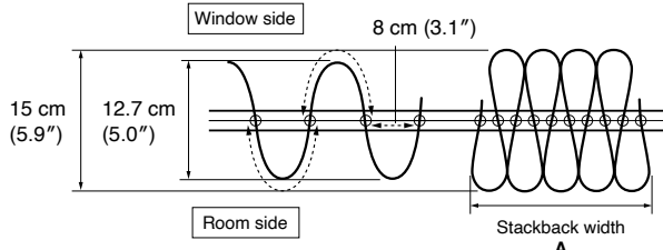
Wave Style Composition of 1.875 Times Fullness
