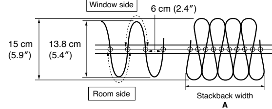
Wave Style Composition of 2.5 Times Fullness
