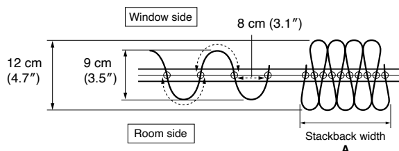
Wave Style Composition of 1.5 Times Fullness
