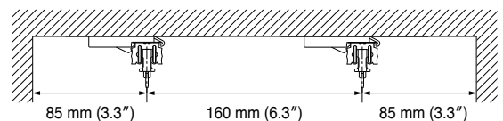
Installation Dimension of 2.5 Times Fullness (example for New Delac)
