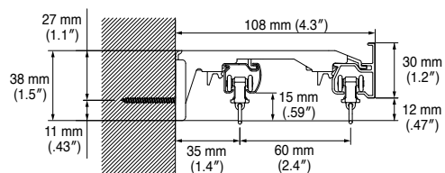
LT Double Bracket * Bracket width = 35 mm (1.4")
