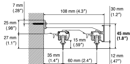
Double Bracket Bracket width = 18 mm (.71")
