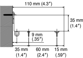
Installation dimension
