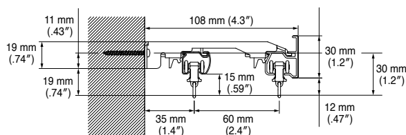
NT Double Bracket * Bracket width = 44 mm (1.7")
