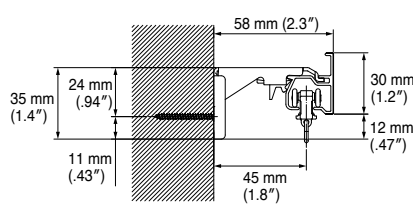
LT Extra Single Bracket * Bracket width = 35 mm (1.4")
