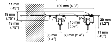
NT Double Bracket Bracket width = 44 mm (1.7")
