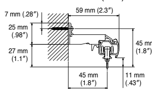
Extra Single Bracket Bracket width = 18 mm (.71")
