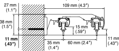
LT Double Bracket Bracket width = 35 mm (1.4")
