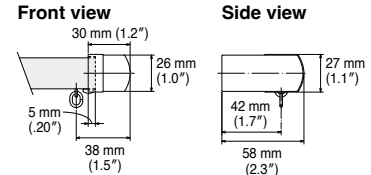
End Cap M (Single)
