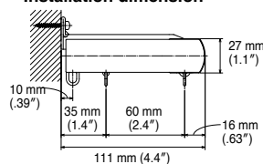
Installation dimension
