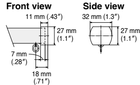
Installation dimension
