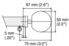
End Cap M (Double)
