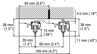
Ceiling Double Bracket Bracket width = 19 mm (.75")
