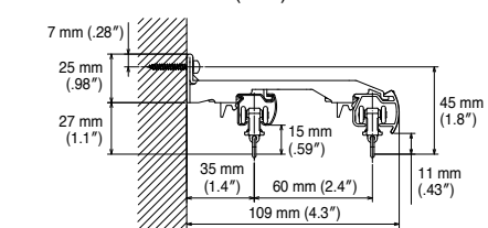
NT Double Bracket Bracket width = 44 mm (1.7")
