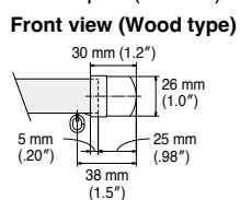
End Cap M (Double)
