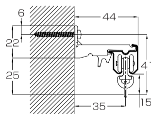
Mounting on a Single Bracket (Bracket width: 18 mm)
