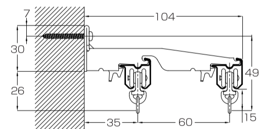
Mounting on a Double Bracket (Bracket width: 18 mm)
