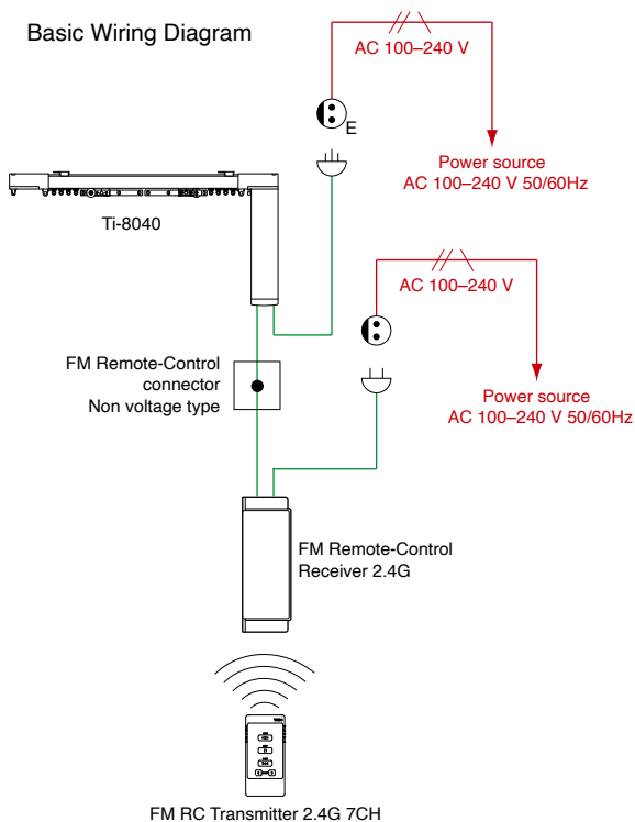
Basic Connecting Diagram
