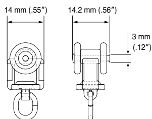
Noiseless Roller
