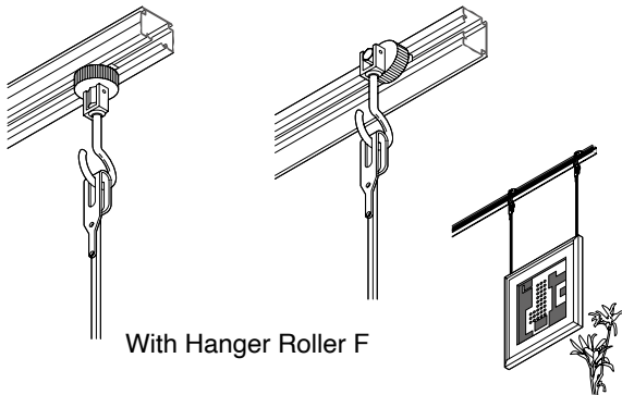
Ceiling Attachment
