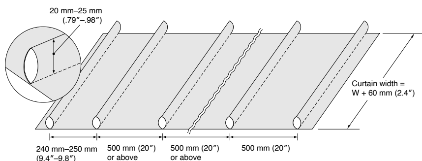
Skylight curtain with Supertrac and Cording Parts Kit for Skylight
