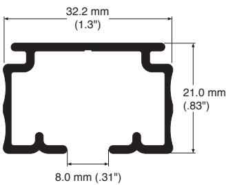
Rail Cross Section
