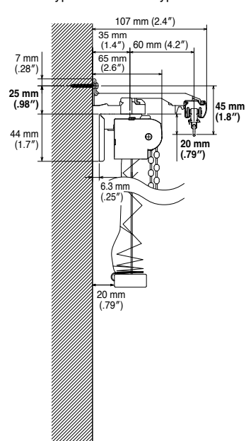
Pleated Blind (SHIORI 25) Chain type / Chain Twin type
