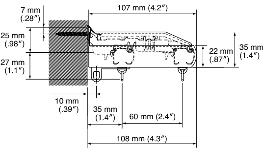
Side view / Cover Top + End Cap M
