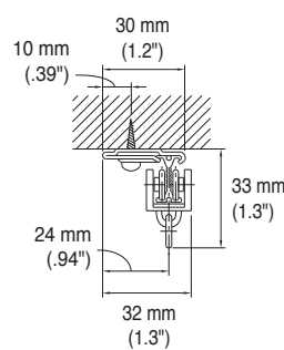
Ceiling Single Bracket Bracket width = 14 mm (.55")
